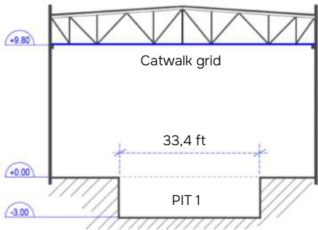
CROSS-SECTION A / A ON PIT 1
